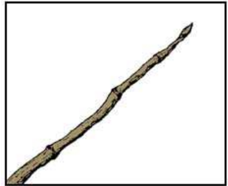
Figure 1. The distance between bud scale scars provides an excellent indication of a tree's growth rate. The ring of scars near the branch tip shows where growth started last spring. The bud scars near the base of the branch denote where the previous season's growth started. By locating bud scars for the past 3 to 4 years the rate of growth can be determined readily.
